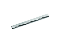
GA550 Galvanised steel rack 22x22x1000 module 4.
